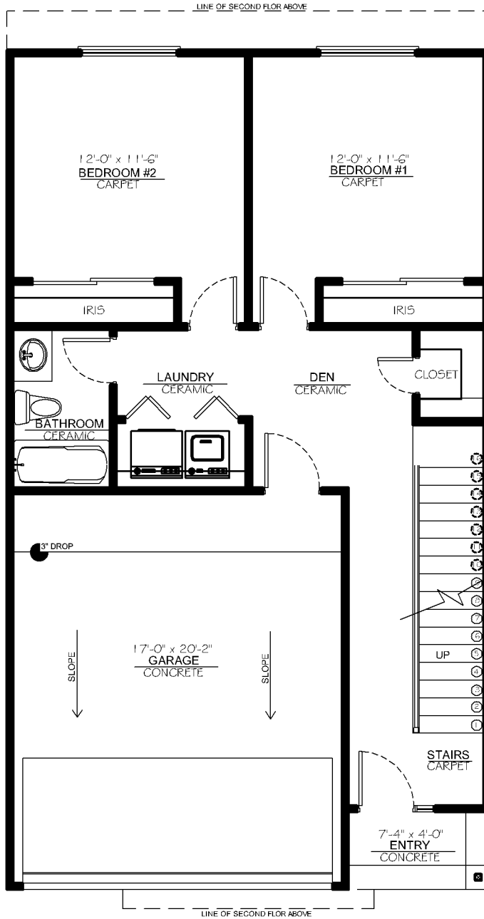
FIRST FLOOR 690 S.F.
